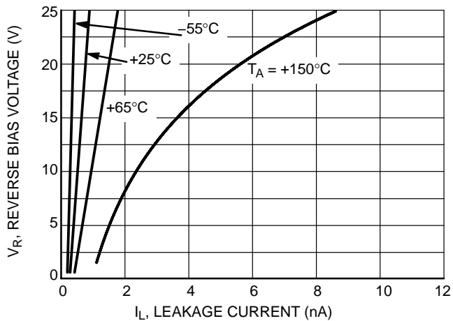
Figure 5. I_R versus Temperature Characteristics of the NUP2105L
