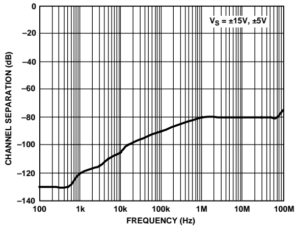
Figure 31. Channel Separation
